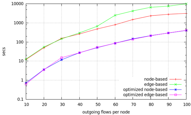
Figure 9: Performance improvement when using the affected subgraph algorithm on structured network overlays with 1000 nodes and different number of outgoing flows per node.
