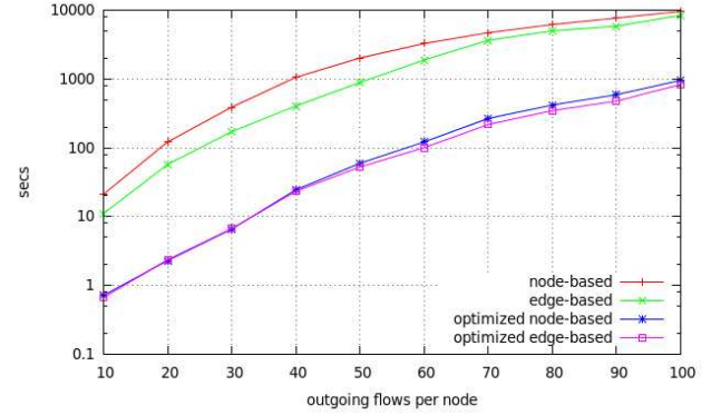
Figure 7: Performance improvement when using the affected subgraph algorithm on random network overlays with 1000 nodes and different number of outgoing flows per node.
