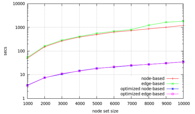
Figure 10: Performance improvement when using the affected subgraph algorithm on structured network overlays with varying size and 20 outgoing flows per node.
