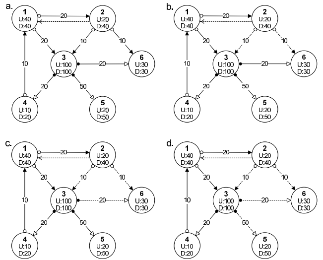
Figure 2: An example of the affected subgraph discovery.
