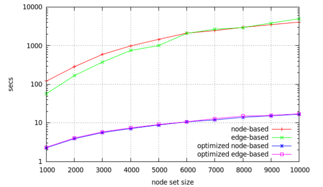
Figure 8: Performance improvement when using the affected subgraph algorithm on random network overlays with varying size and 20 outgoing flows per node.
